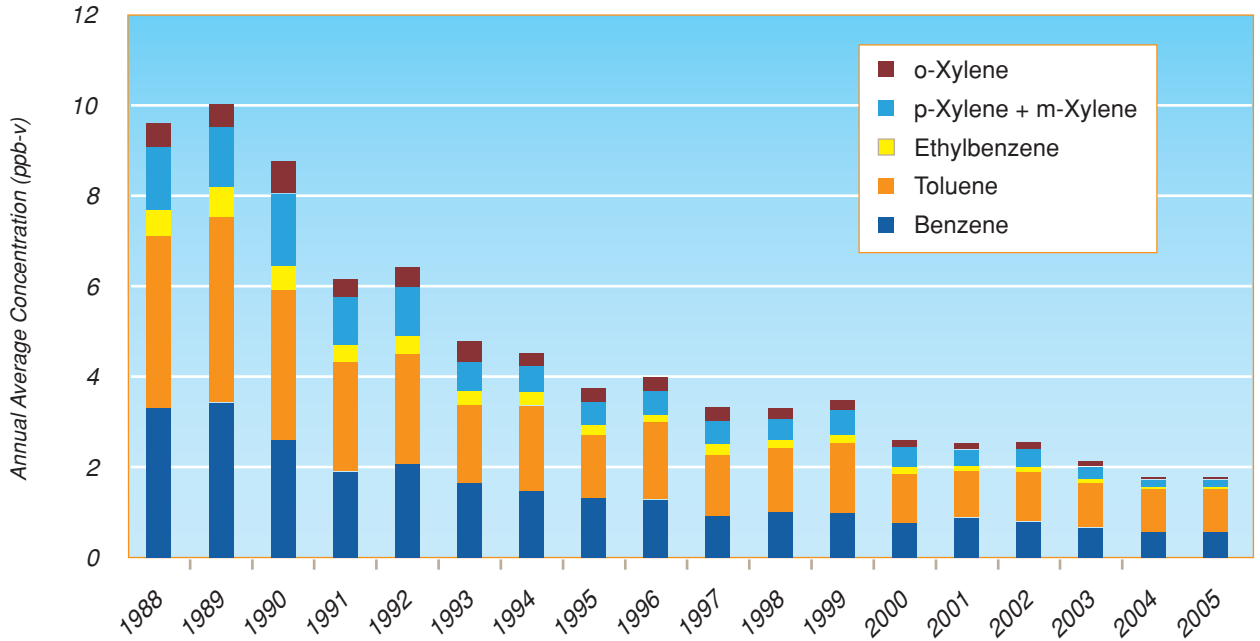
Annual Average Trends for BTEX for HRM Network from 1988 through 2005
